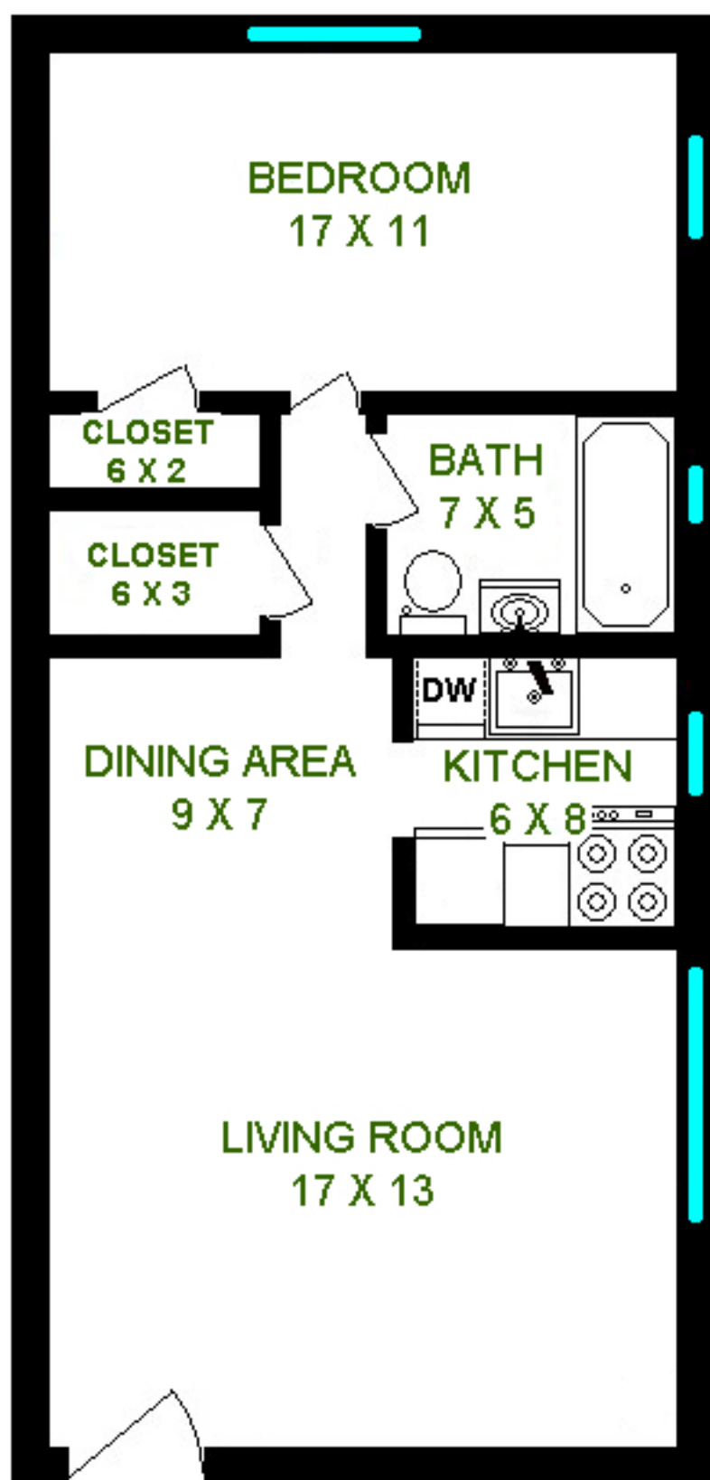
KINGSFORD- Spruce One Bedroom- 630 sq. ft. Sizes and proportions are approximate.
